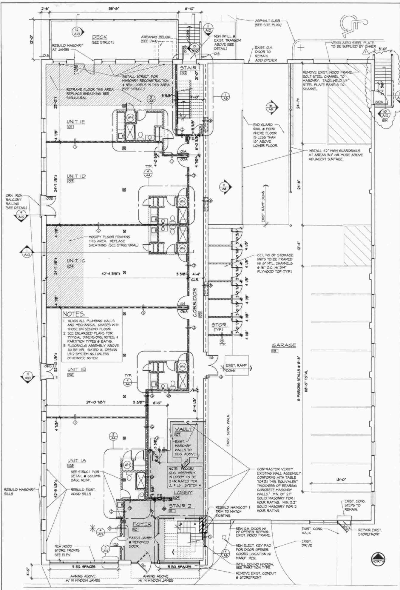
2 FIRST FLOOR PLAN
